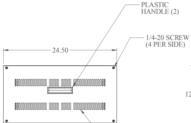
L.S. VIEW
