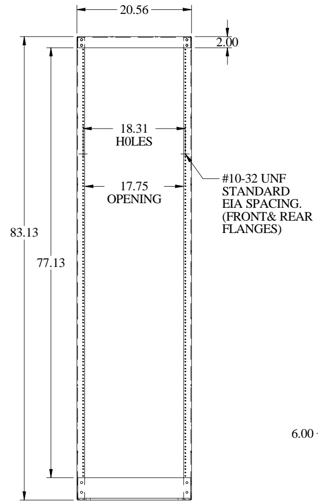
FRONT VIEW
