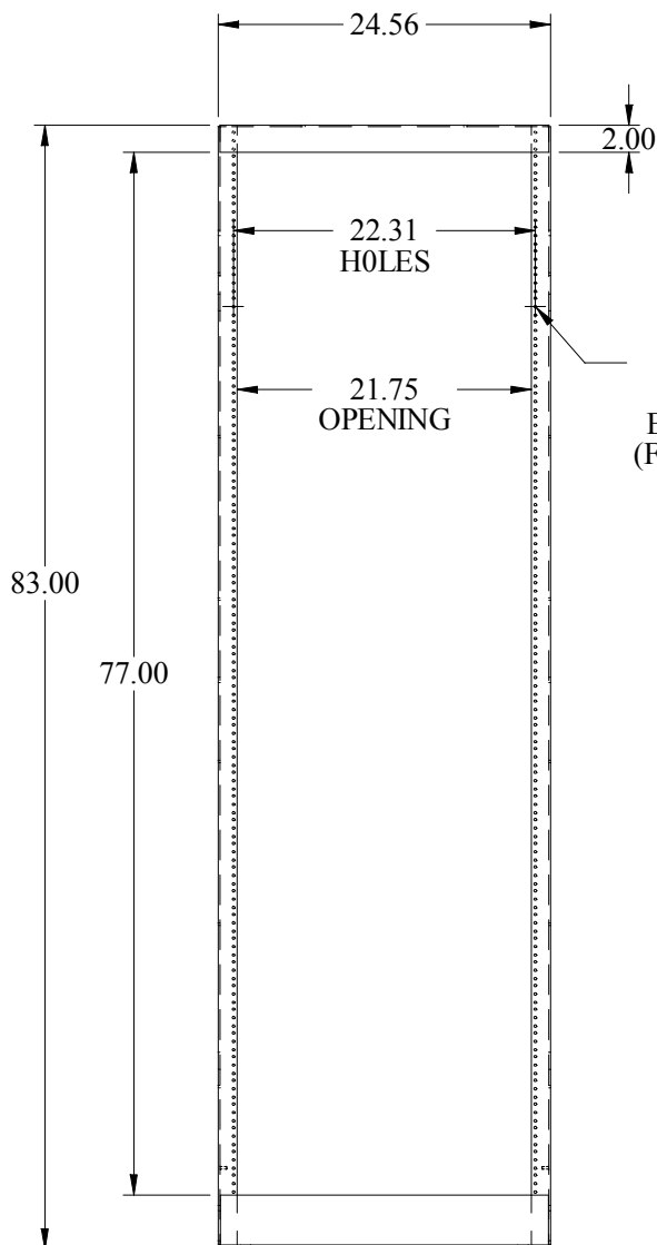
FRONT VIEW
