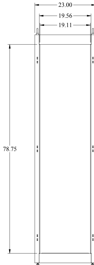
FRONT VIEW
