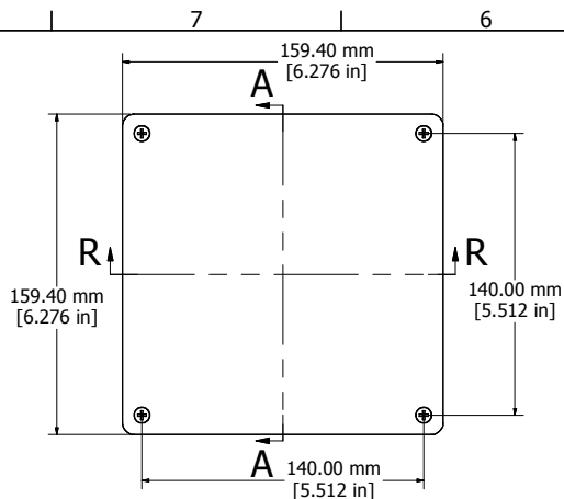
ASSEMBLY
