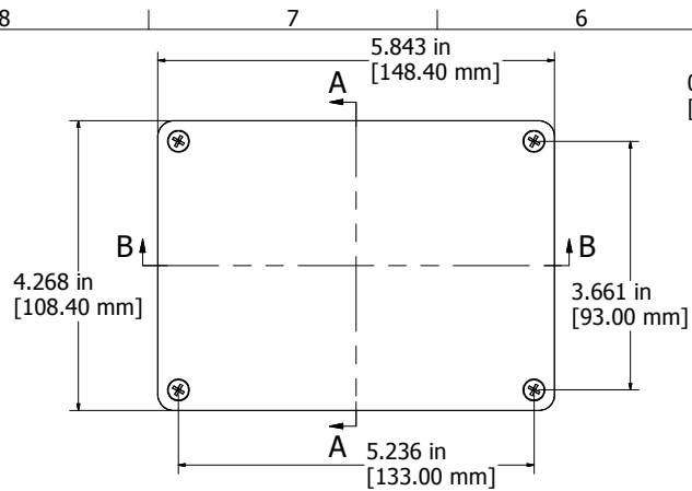
ASSEMBLY
