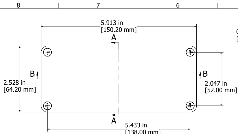
ASSEMBLY
