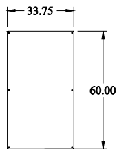
INNER PANEL
