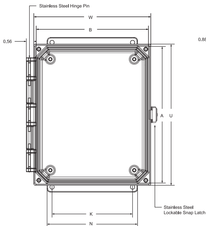
Front View
