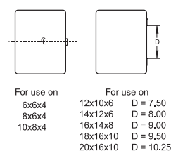
Latch Locations
