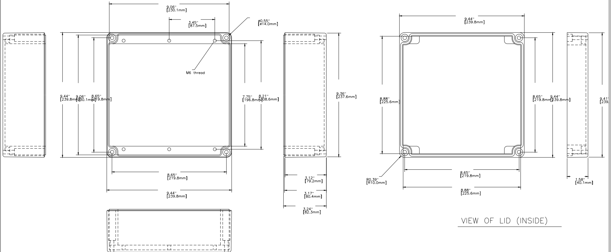
VIEW OF BOX (LID REMOVED)
