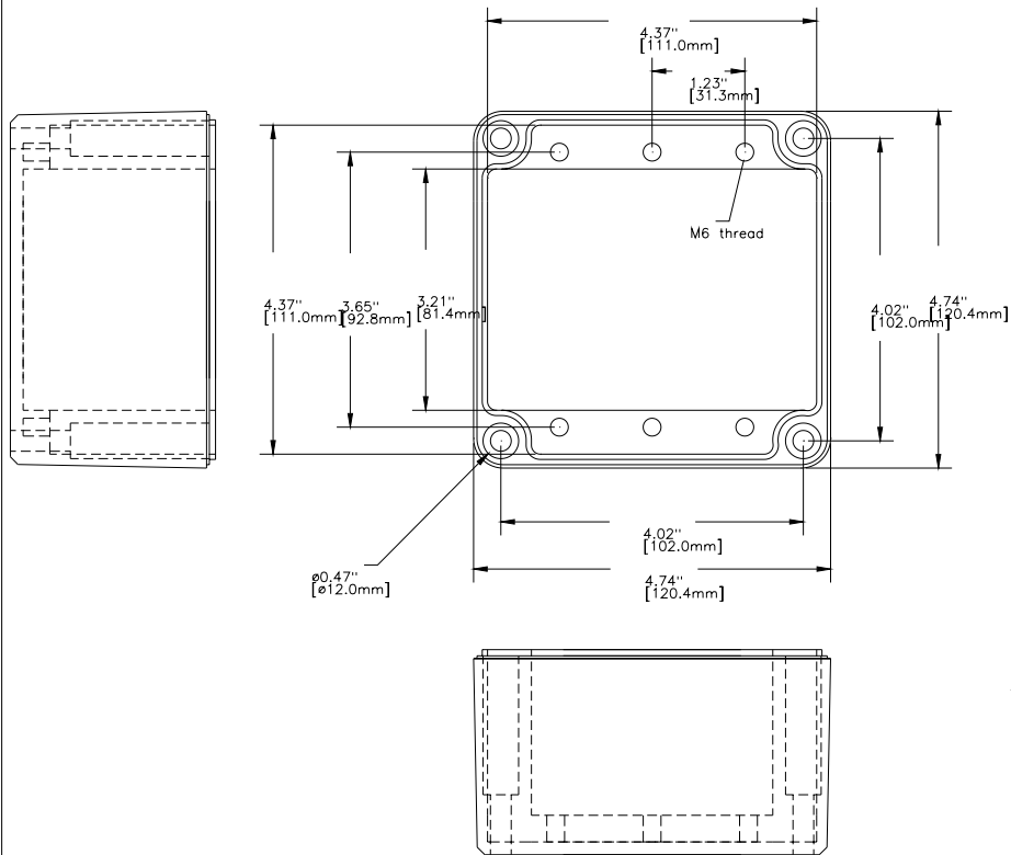
VIEW OF BOX (LID REMOVED)
