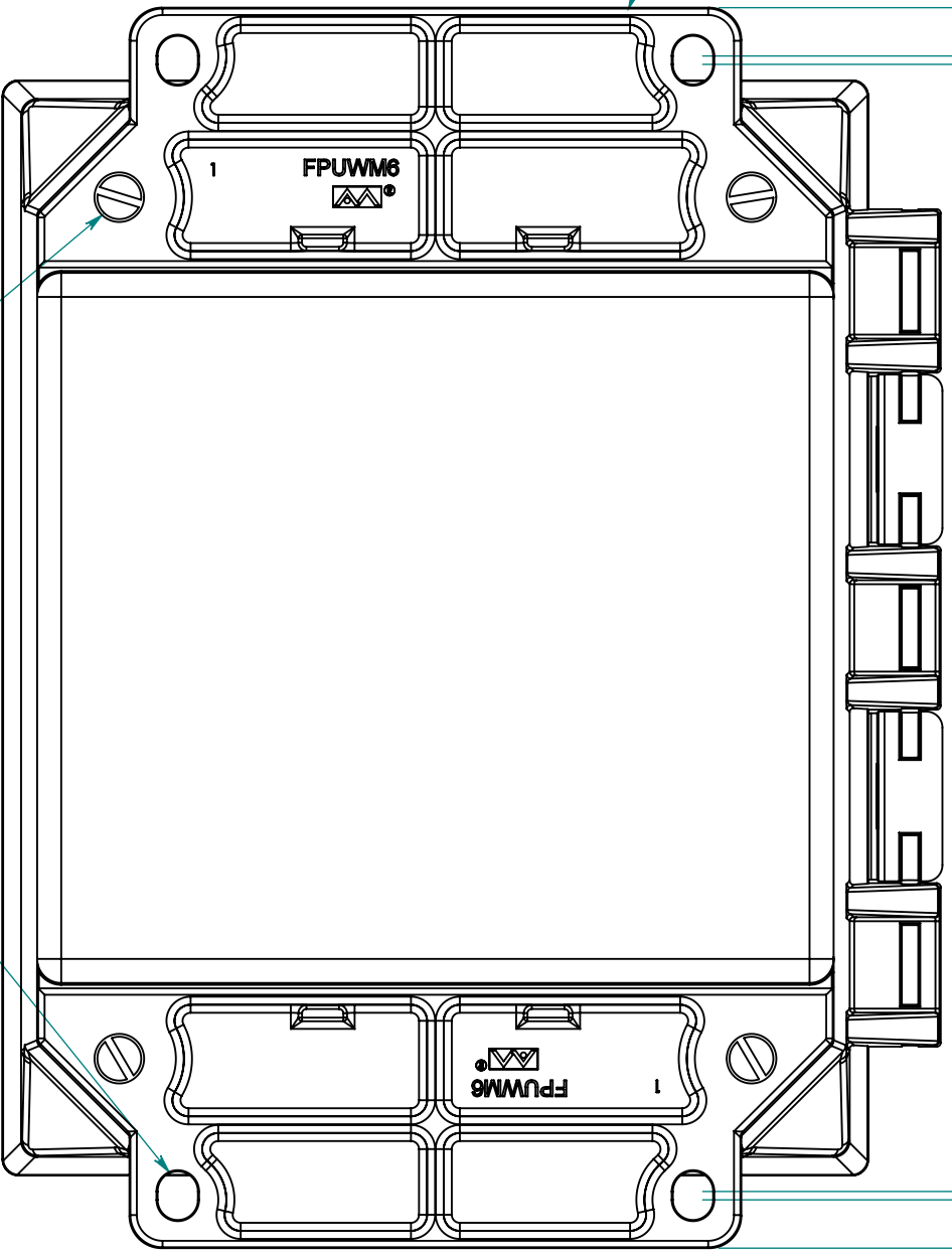
BACK VIEW
