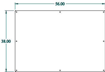
INNER PANEL
