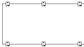
BACK VIEW
