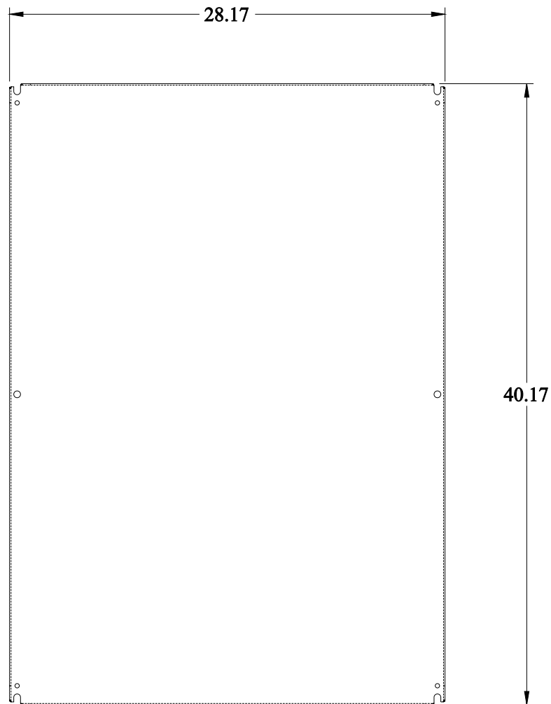
FRONT VIEW
