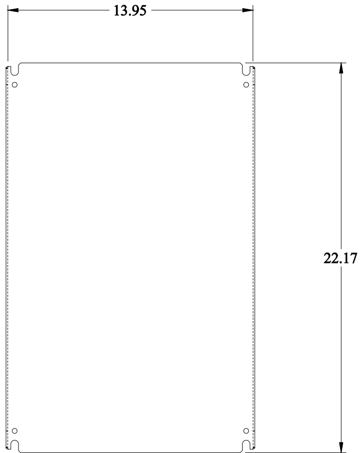
FRONT VIEW
