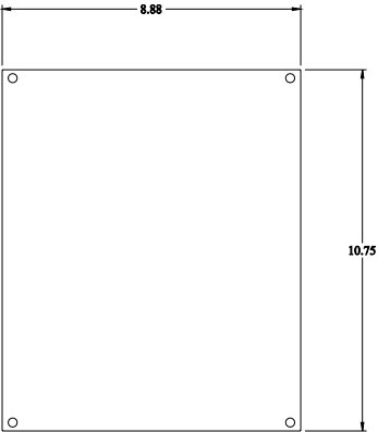
INNER PANEL
