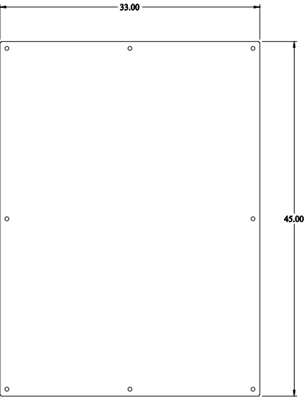
INNER PANEL
