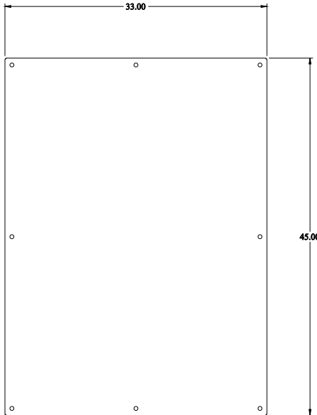
INNER PANEL
