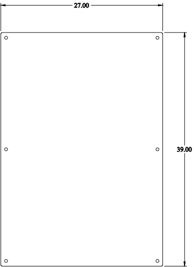
INNER PANEL
