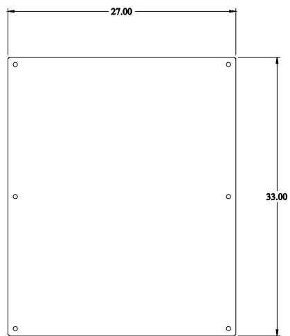
INNER PANEL
