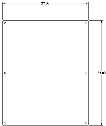
INNER PANEL
