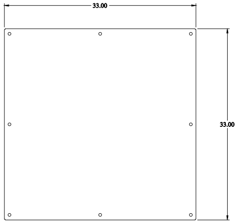
INNER PANEL
