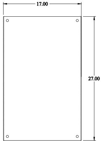
INNER PANEL
