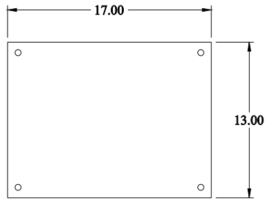
INNER PANEL
