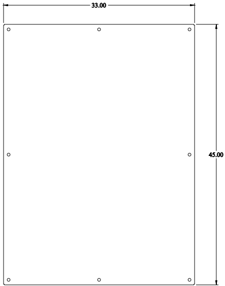
INNER PANEL
