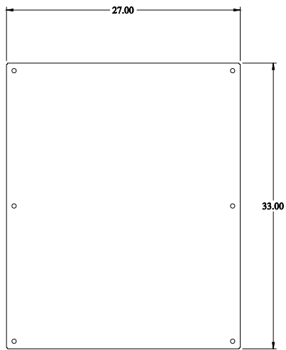
INNER PANEL
