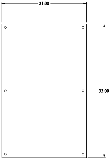
INNER PANEL
