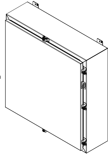
ISOMETRIC VIEW
