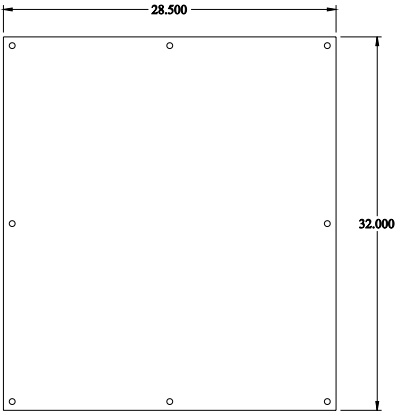
INNER PANEL
