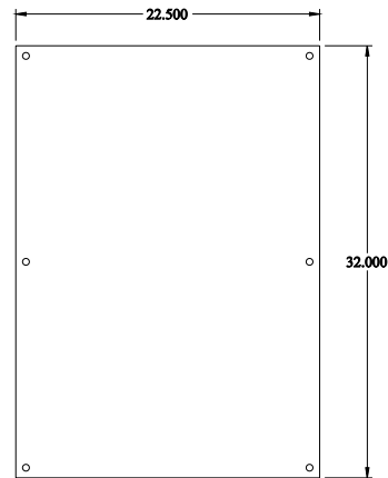
INNER PANEL
