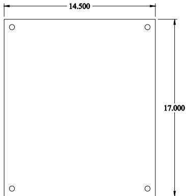
INNER PANEL
