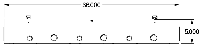
FRONT VIEW
