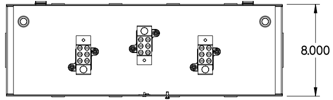
TOP VIEW - COVER REMOVED
