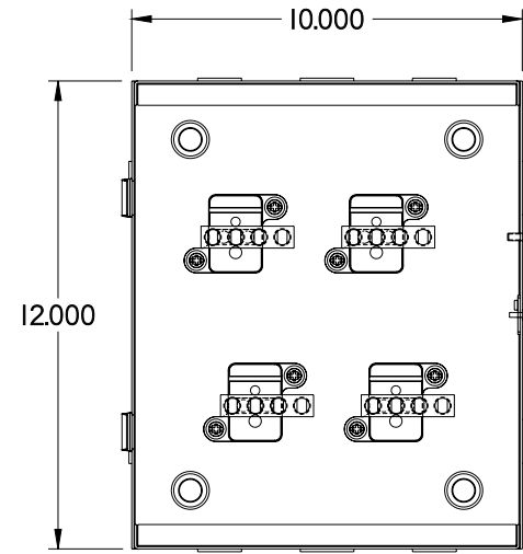
FRONT VIEW - COVER REMOVED
