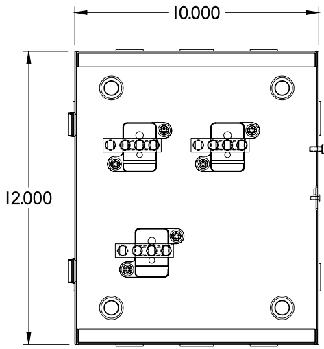
FRONT VIEW - COVER REMOVED
