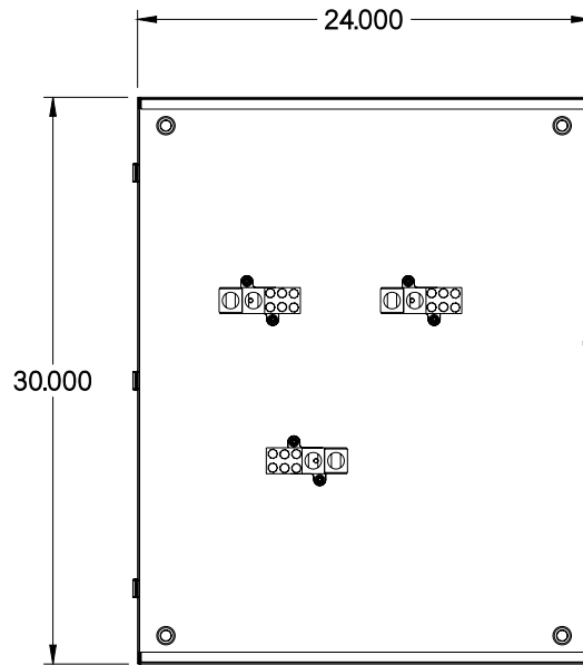
FRONT VIEW - COVER REMOVED
