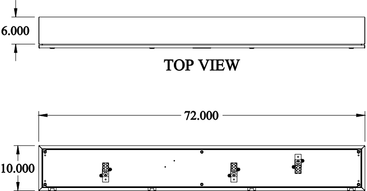
FRONT VIEW - COVER REMOVED
