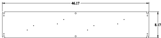
INNER PANEL
