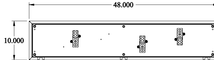
FRONT VIEW - COVER REMOVED
