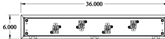
FRONT VIEW - COVER REMOVED
