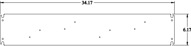
INNER PANEL
