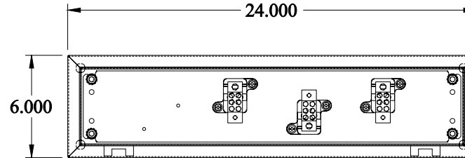
FRONT VIEW - COVER REMOVED
