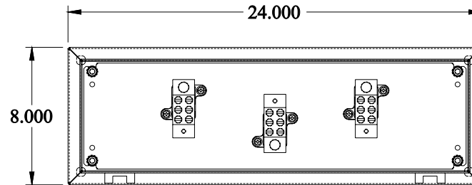
FRONT VIEW - COVER REMOVED
