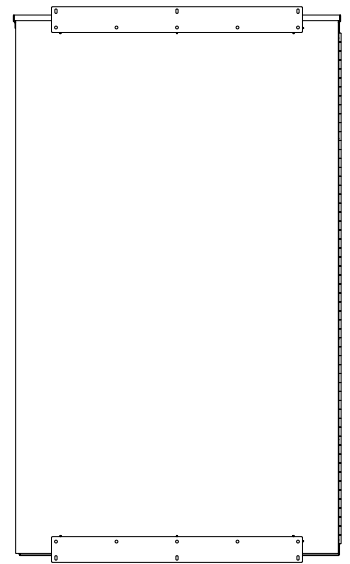
BACK VIEW
