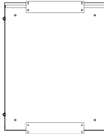
BACK VIEW
