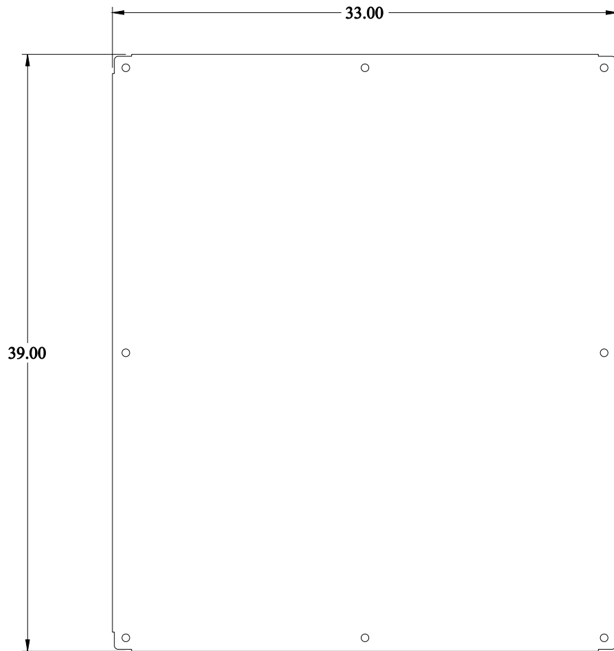
FRONT VIEW
