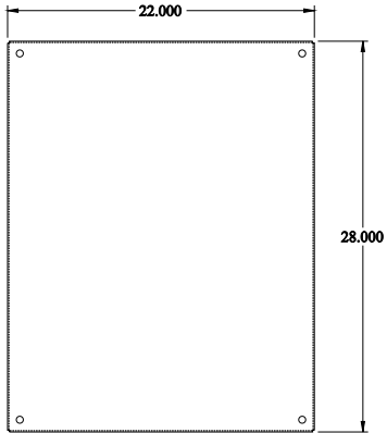
INNER PANEL
